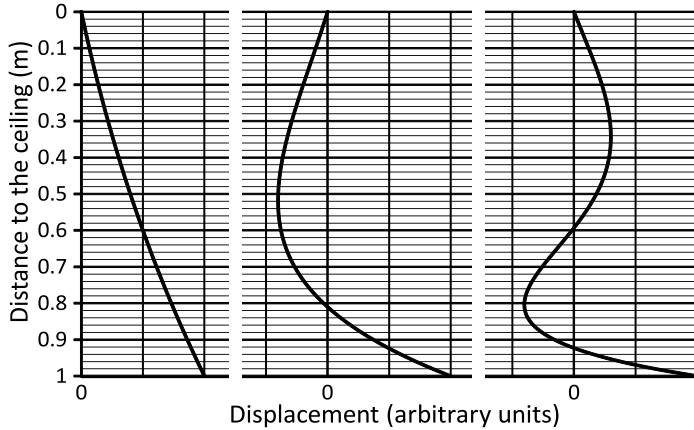
Figure: Shapes of the oscillating rope for the first three natural vibrations ( i = 1, 2, 3 from left to right)
